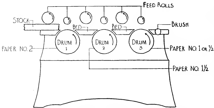
FIG. 203. SECTIONAL VIEW OF DRUM SANDER.
